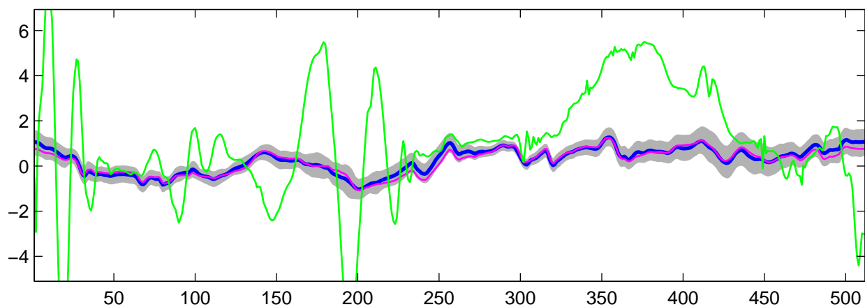
Estimated C_1(t) using R-WFMM: t_1 data, run 2
