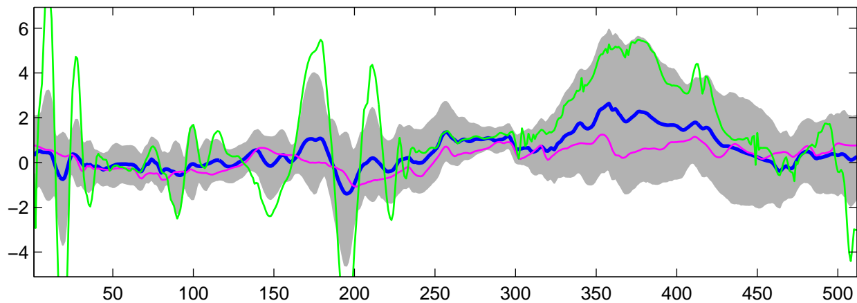
Estimated C_1(t) using G-WFMM: t_1 data, run 2
