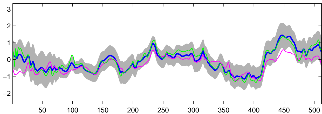
Estimated C_2(t) using R-WFMM: DE data, run 2
