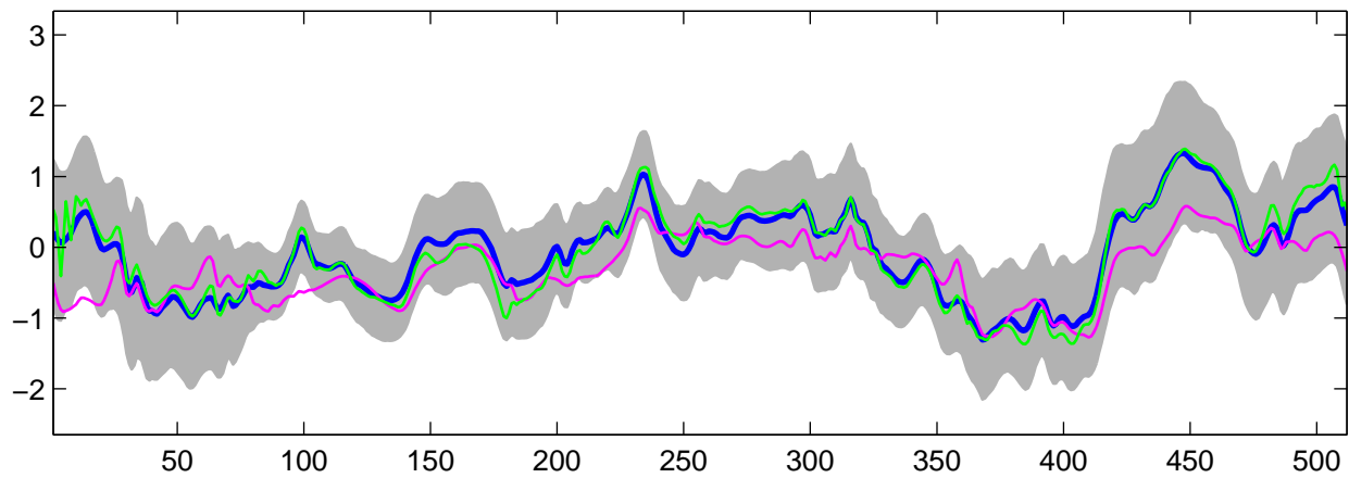
Estimated C_2(t) using G-WFMM: DE data, run 2
