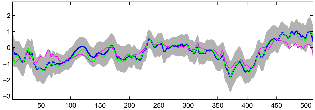
Estimated C_2(t) using G-WFMM: Normal data, run 2
