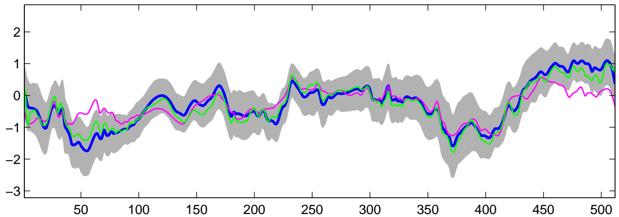
Estimated C_2(t) using R-WFMM: Normal data, run 2
