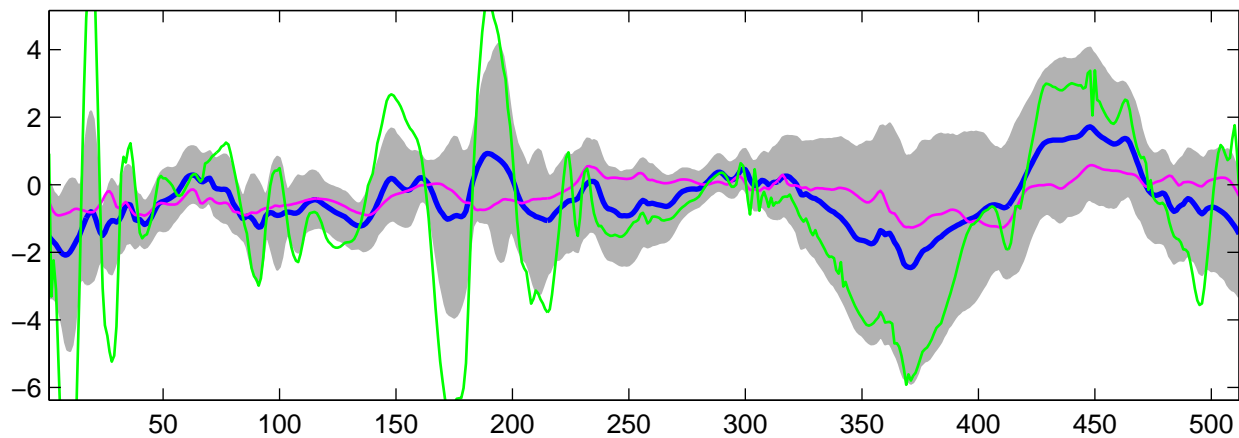
Estimated C_2(t) using G-WFMM: t_1 data, run 2
