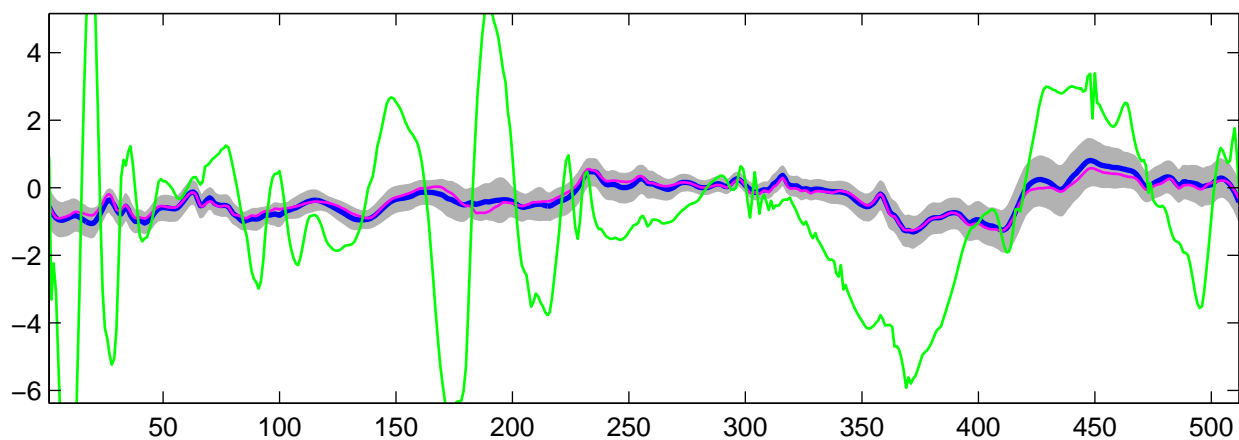
Estimated C_2(t) using R-WFMM: t_1 data, run 2
