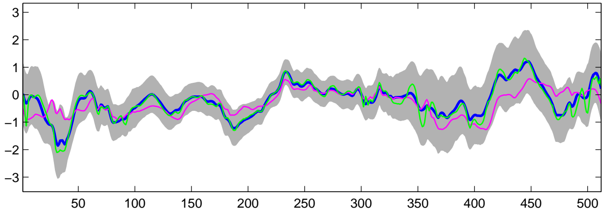
Estimated C_2(t) using G-WFMM: t_2 data, run 2
