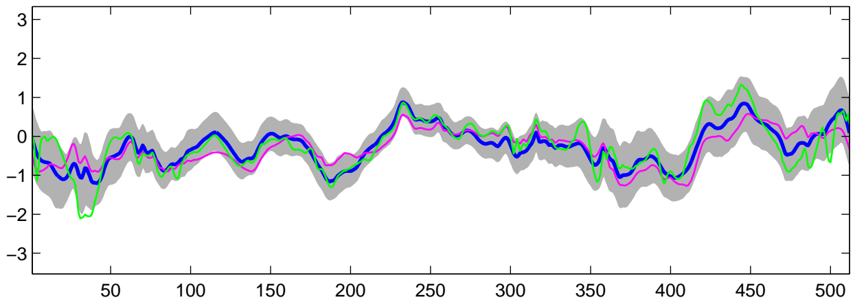
Estimated C_2(t) using R-WFMM: t_2 data, run 2
