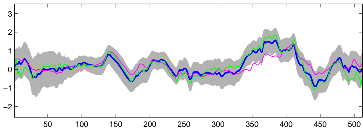
Estimated C_3(t) using R-WFMM: DE data, run 2
