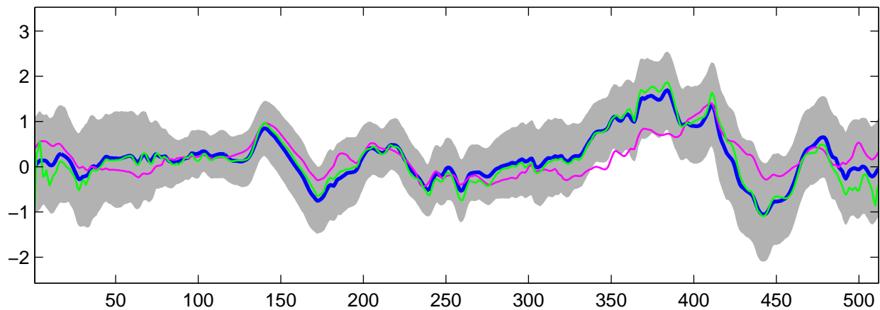
Estimated C_3(t) using G-WFMM: DE data, run 2
