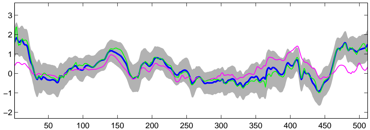
Estimated C_3(t) using R-WFMM: Normal data, run 2
