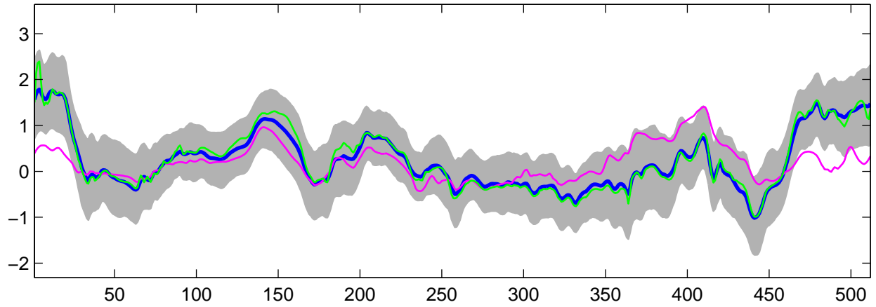
Estimated C_3(t) using G-WFMM: Normal data, run 2
