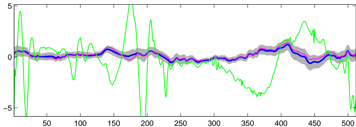
Estimated C_3(t) using R-WFMM: t_1 data, run 2
