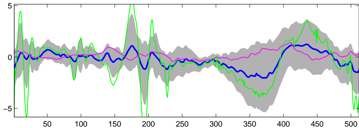
Estimated C_3(t) using G-WFMM: t_1 data, run 2
