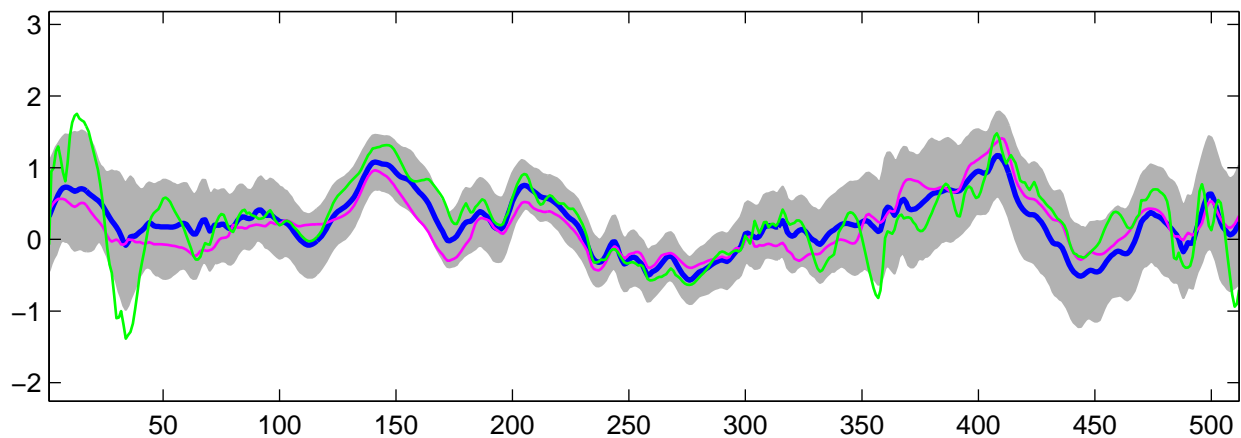
Estimated C_3(t) using R-WFMM: t_2 data, run 2
