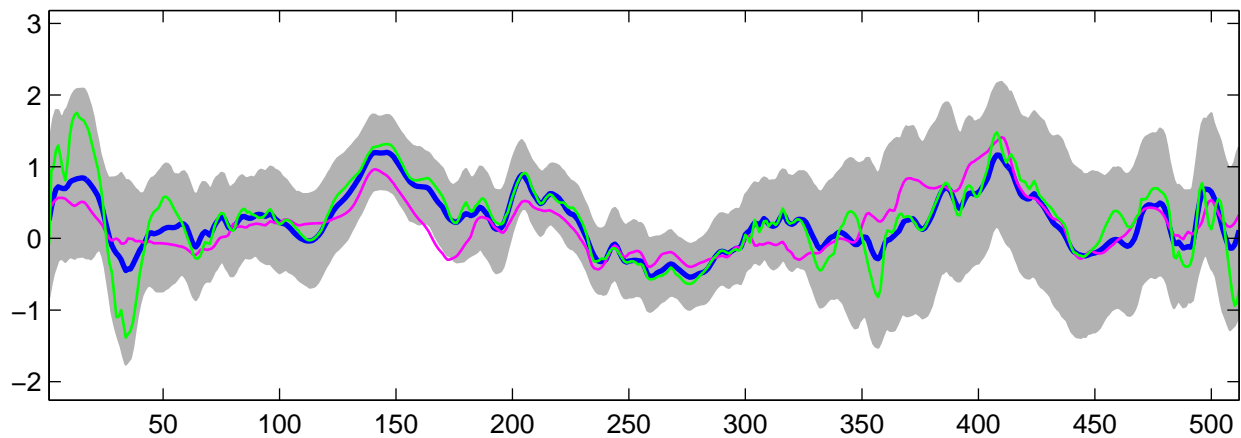
Estimated C_3(t) using G-WFMM: t_2 data, run 2
