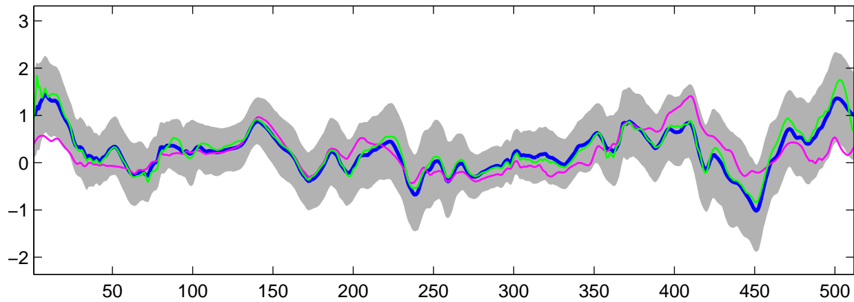
Estimated C_3(t) using G-WFMM: t_3 data, run 2
