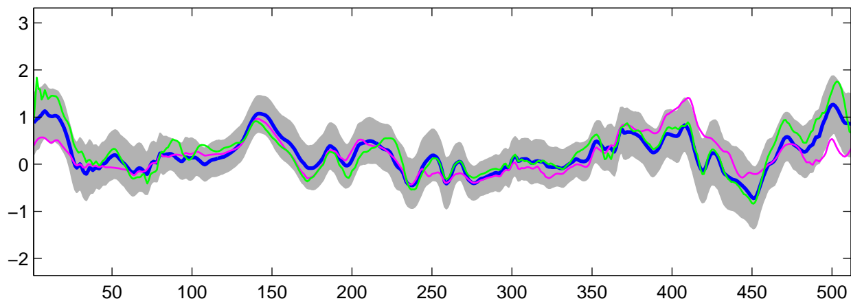
Estimated C_3(t) using R-WFMM: t_3 data, run 2
