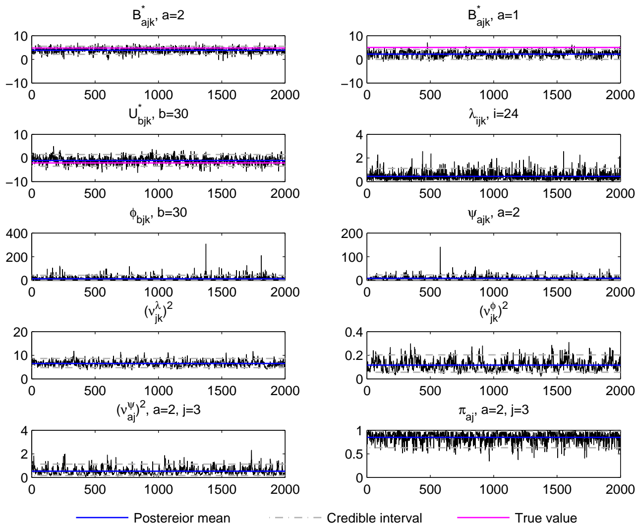
Trace plot, j=3, k=1 , DE data, simulation run 2
