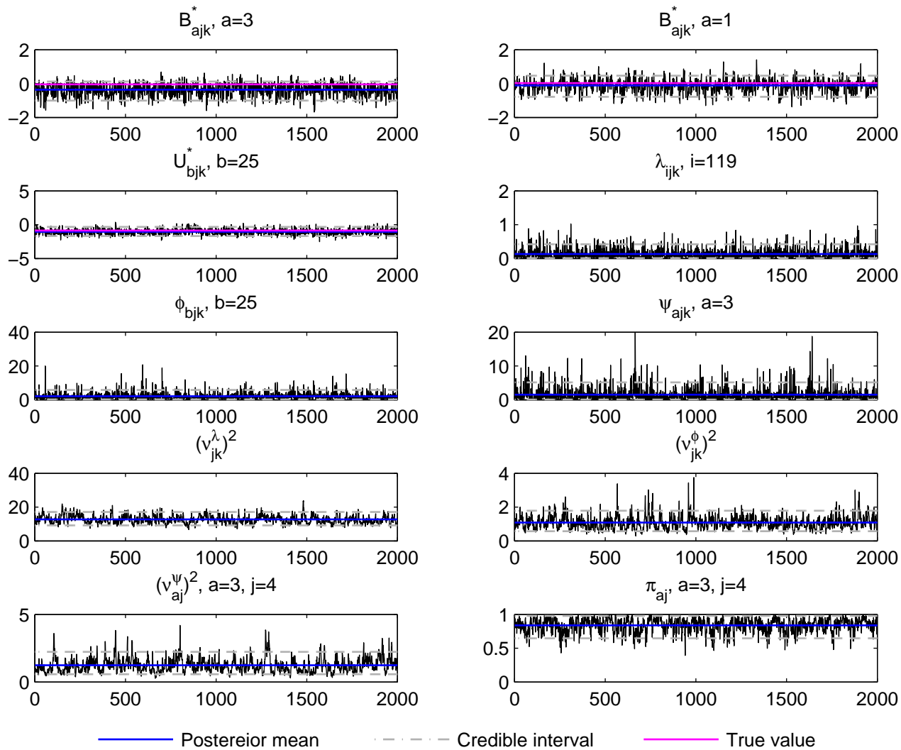
Trace plot, j=4, k=1 , Normal data, simulation run 2
