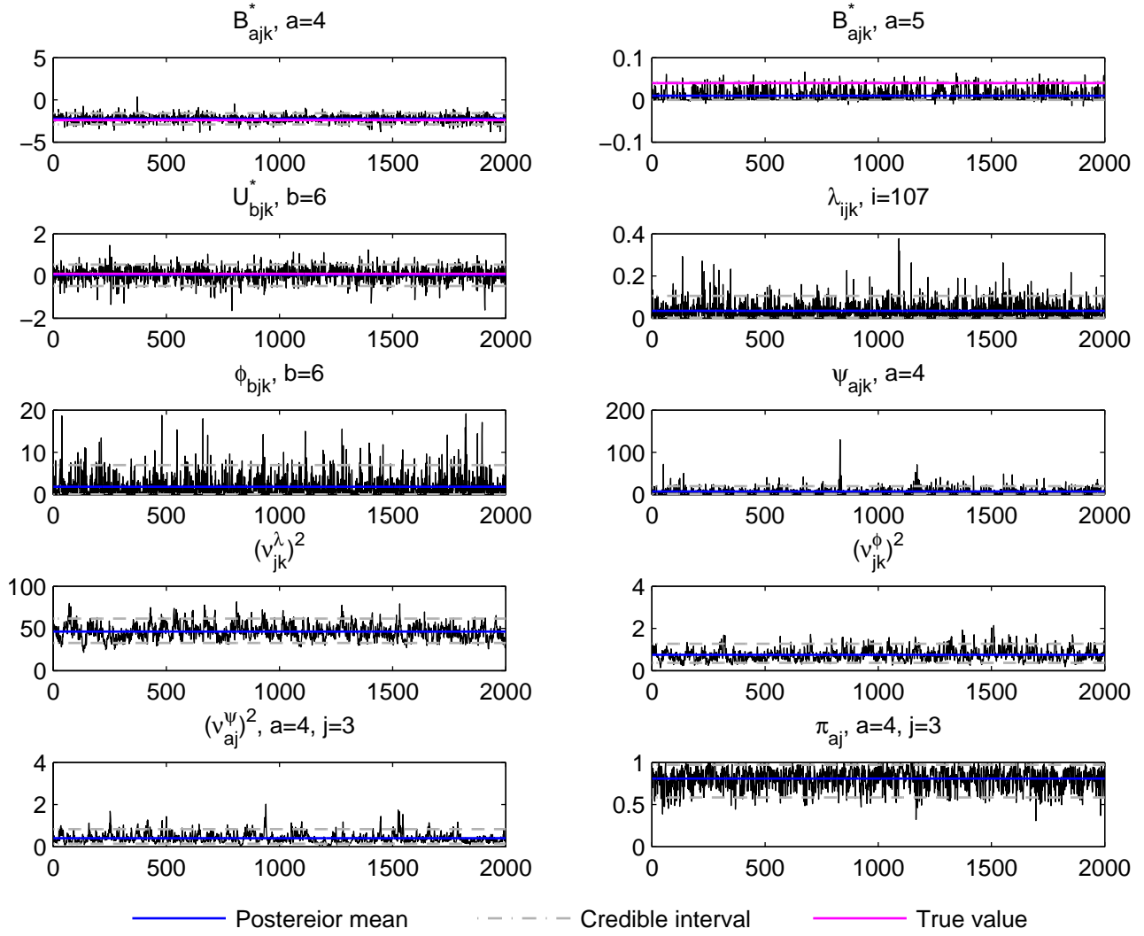
Trace plot, j=3, k=3, t_i data, simulation run 2
