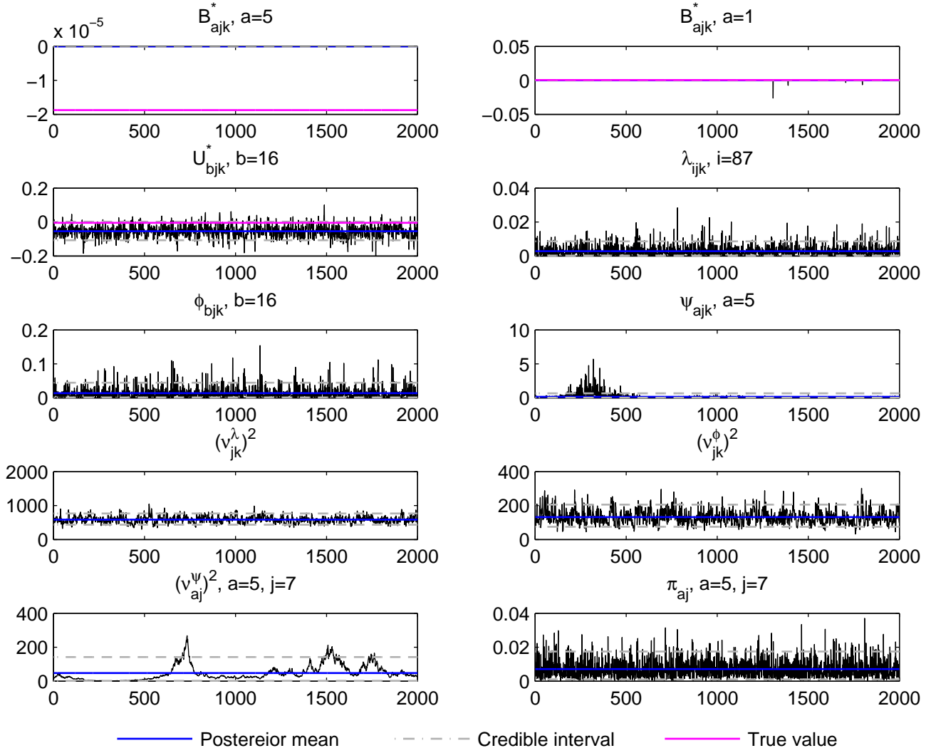
Trace plot, j=7, k=1, t_3 data, simulation run 2
