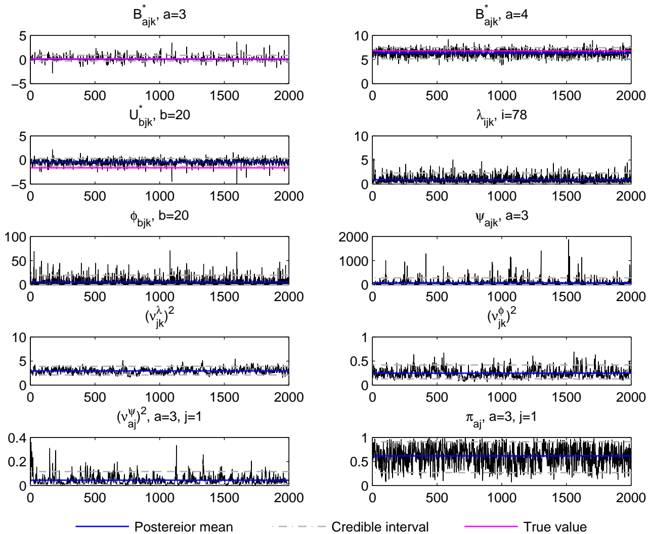
Trace plot, j=1, k=6 , DE data, simulation run 2
