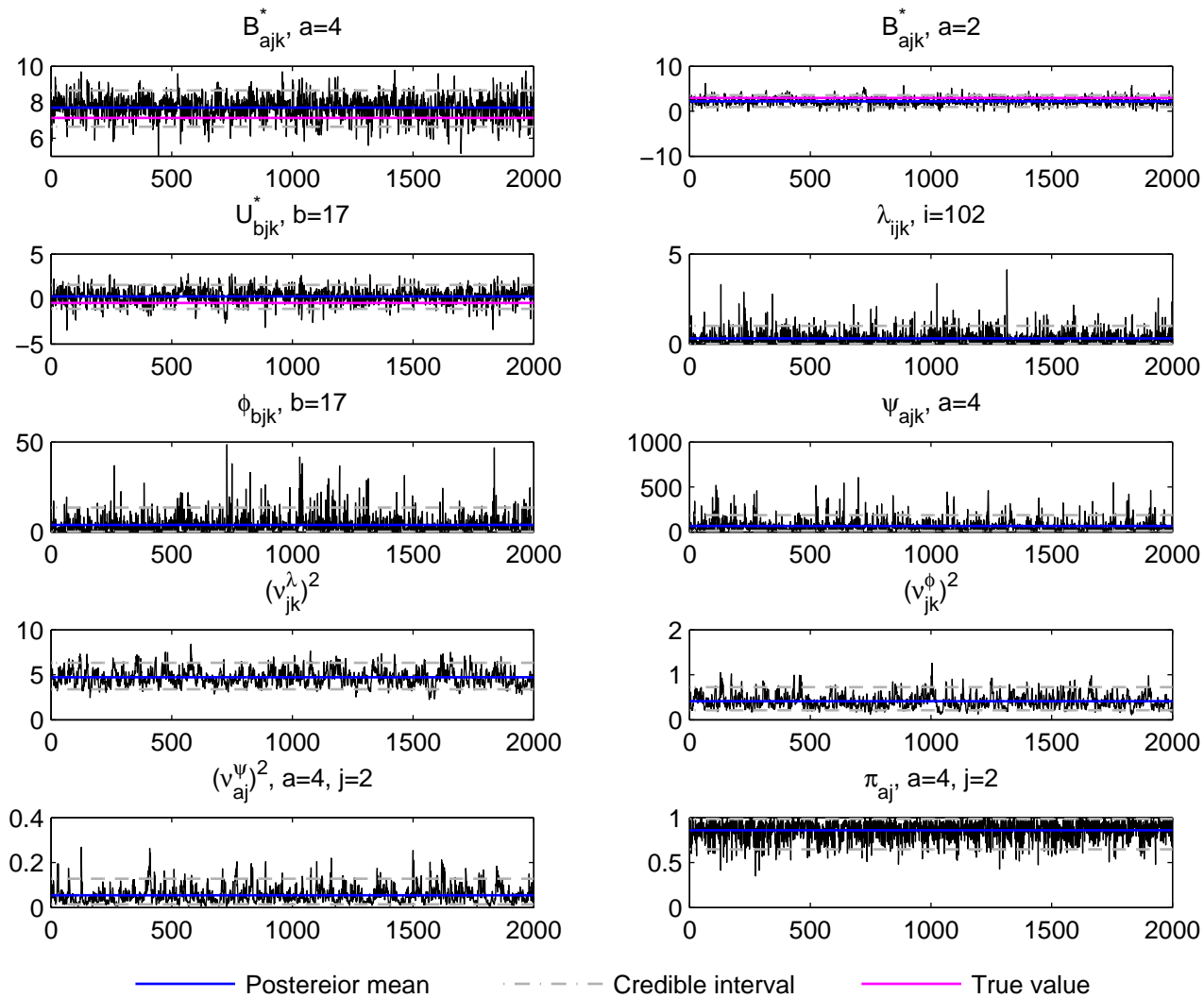
Trace plot, j=2, k=5 , Normal data, simulation run 2
