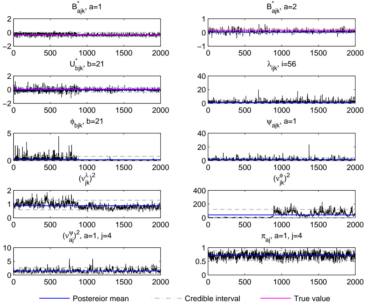
Trace plot, j=4, k=2, t_j data, simulation run 2
