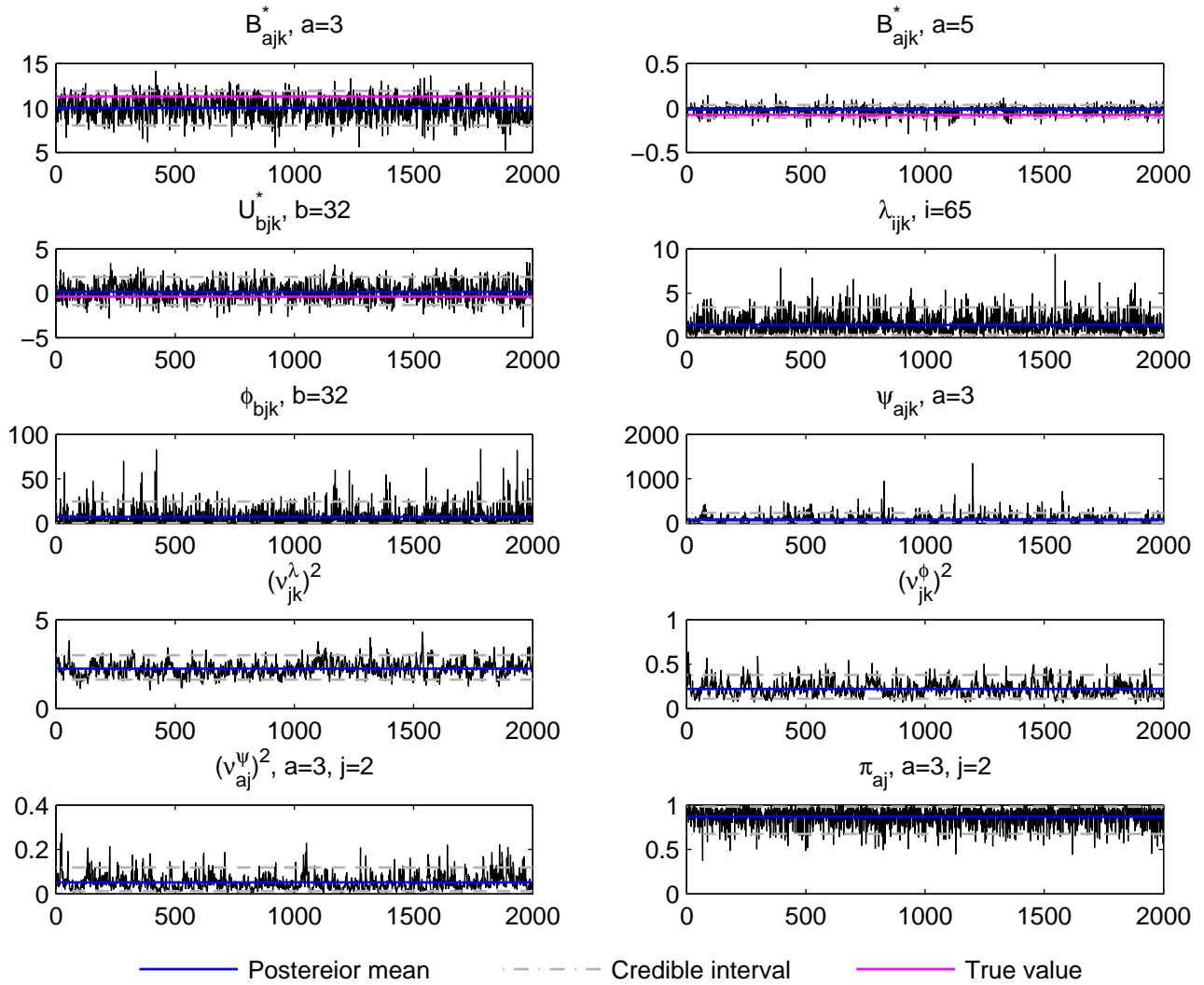
Trace plot, j=2, k=3, t_2 data, simulation run 2
