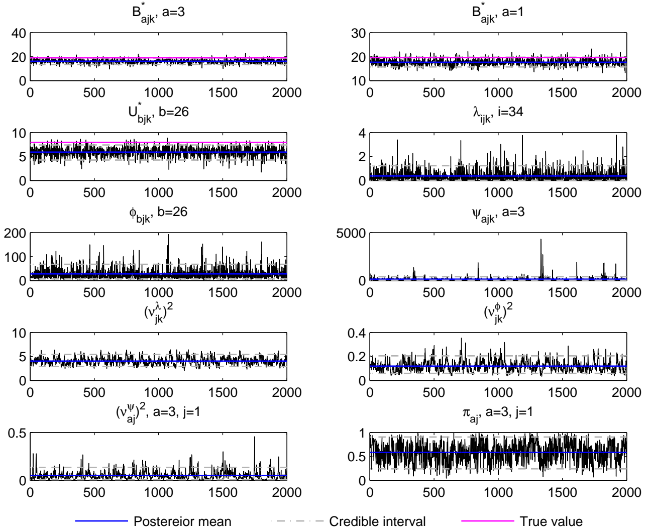
Trace plot, j=1, k=1, t_3 data, simulation run 2
