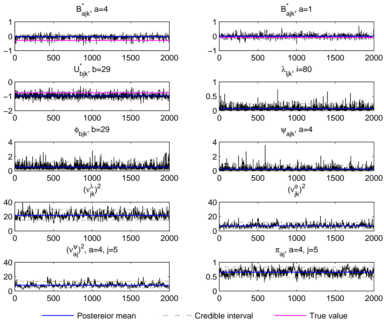
Trace plot, j=5, k=1 , Normal data, simulation run 2
