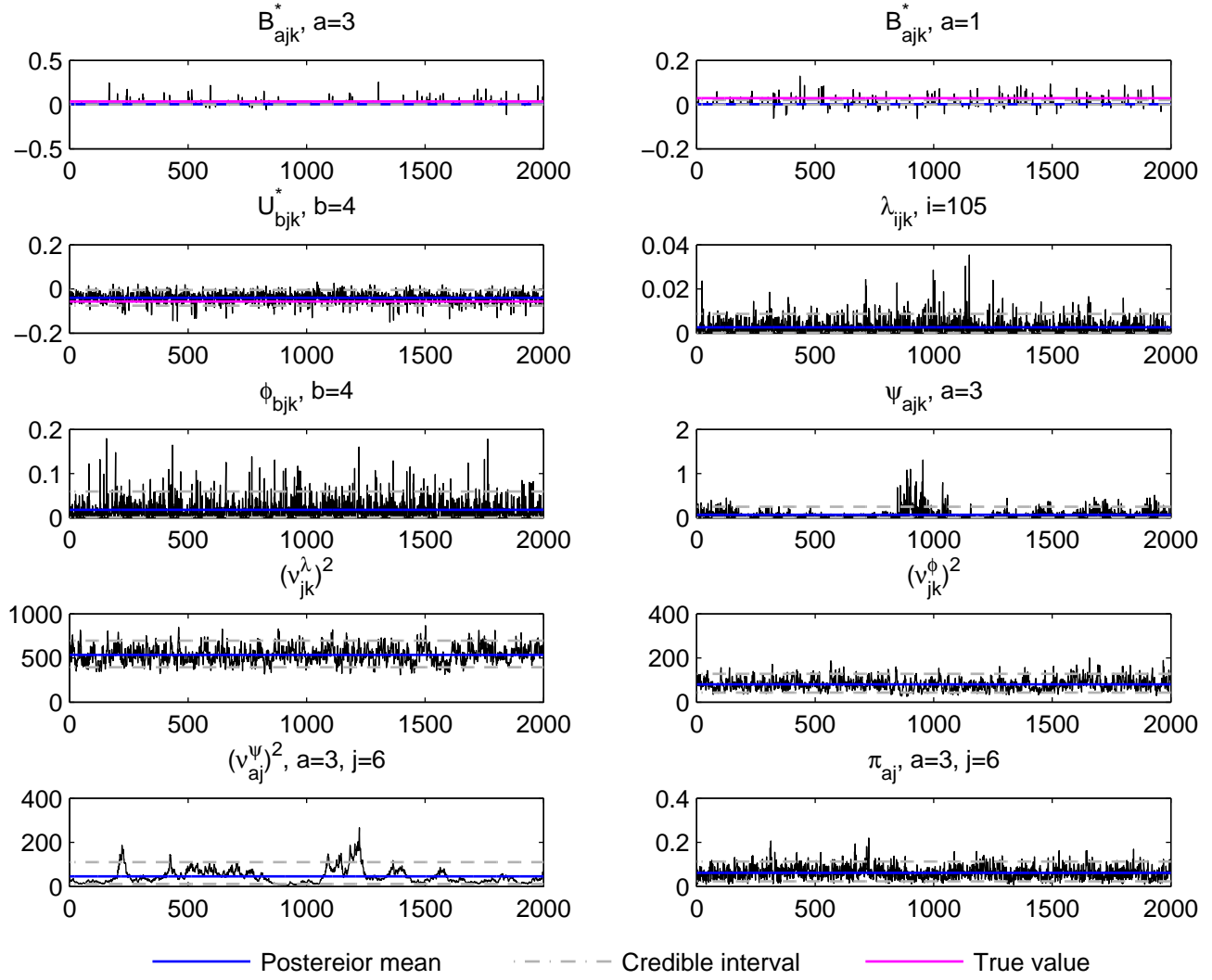
Trace plot, j=6, k=2, t_2 data, simulation run 2
