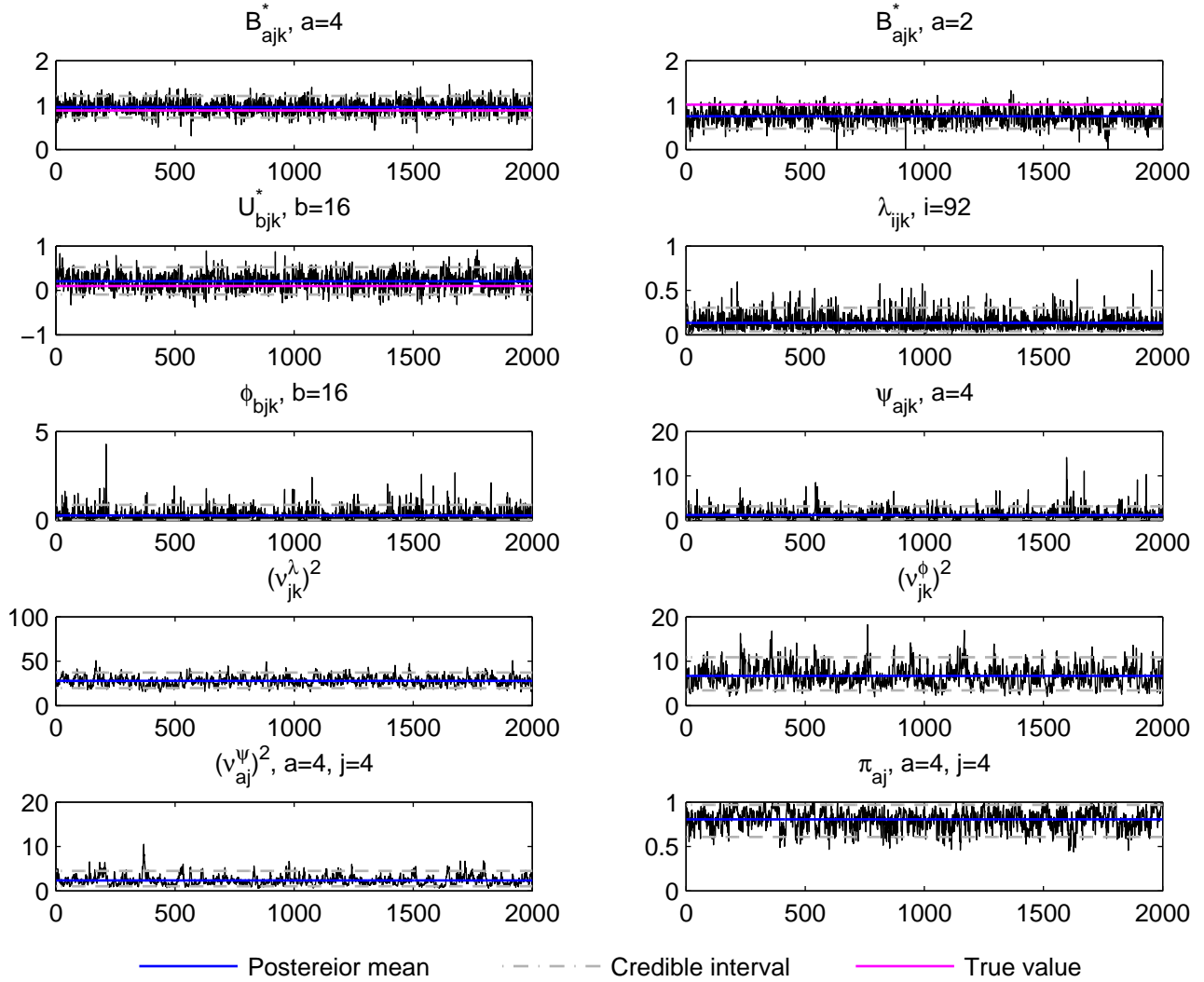
Trace plot, j=4, k=3, t_3 data, simulation run 2
