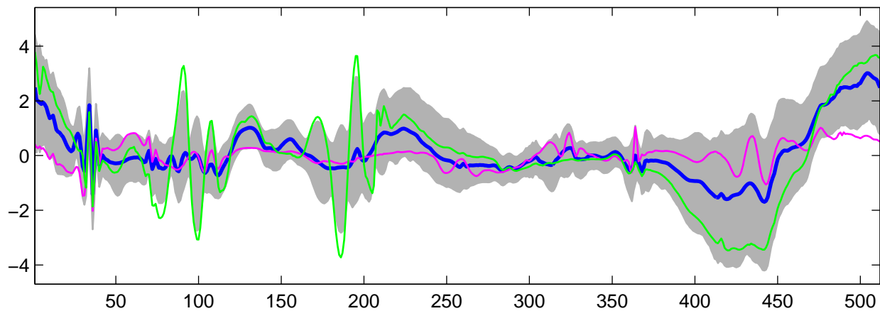
Estimated U_{10}(t) using G-WFMM: t_1 data, run 2
