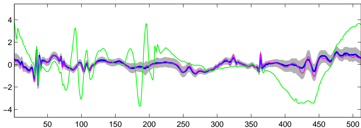
Estimated U_{10}(t) using R-WFMM: t_1 data, run 2
