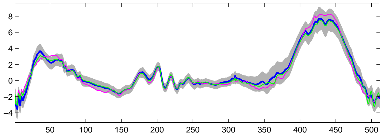
Estimated U_{10}(t) using G-WFMM: t_2 data, run 2
