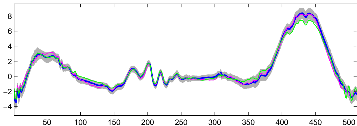
Estimated U_{10}(t) using R-WFMM: t_2 data, run 2
