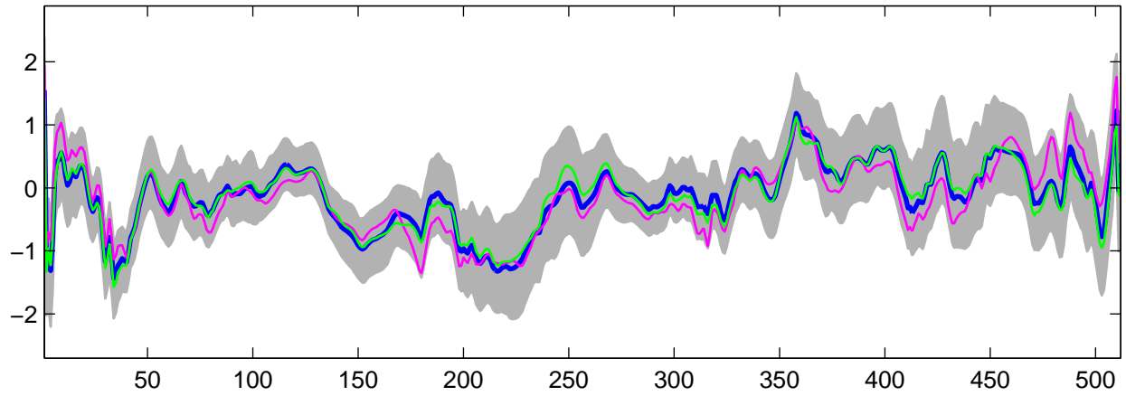
Estimated U_{10}(t) using G-WFMM: t_3 data, run 2
