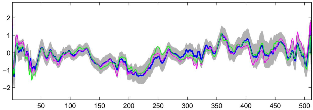
Estimated U_{10}(t) using R-WFMM: t_3 data, run 2
