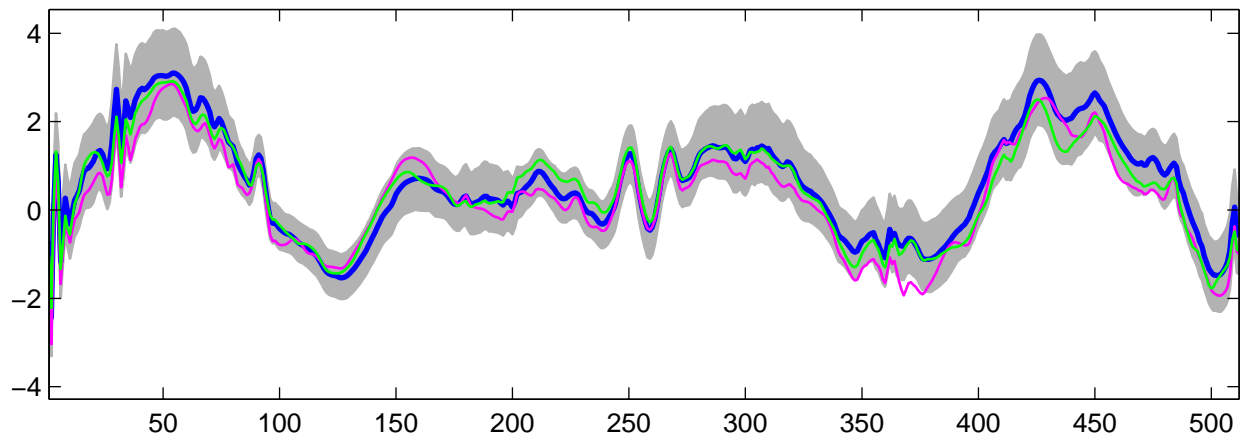
Estimated U_{11}(t) using R-WFMM: DE data, run 2
