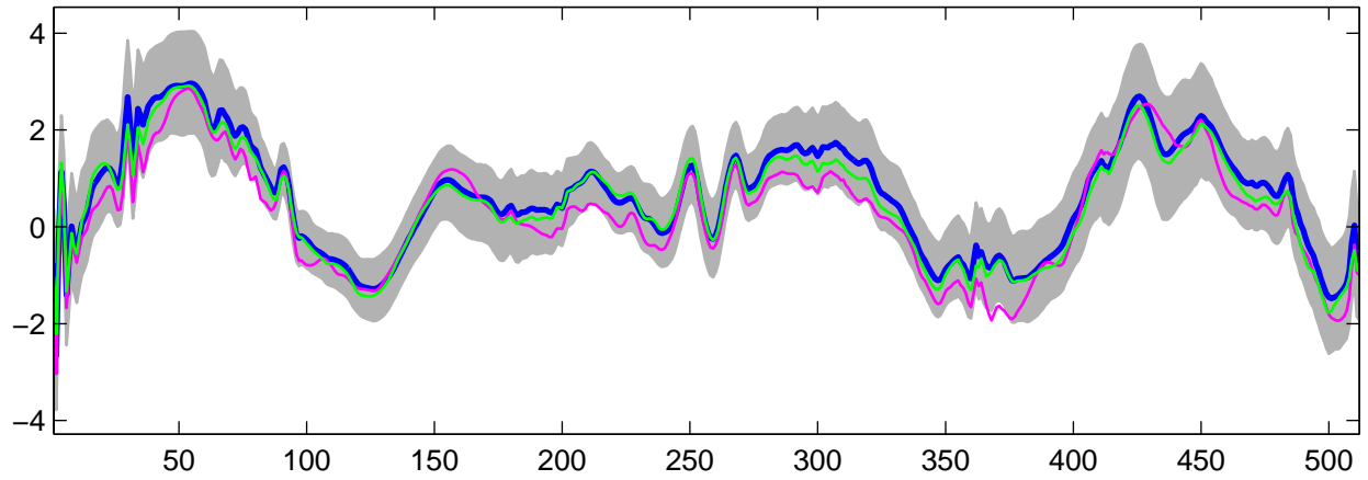
Estimated U_{11}(t) using G-WFMM: DE data, run 2
