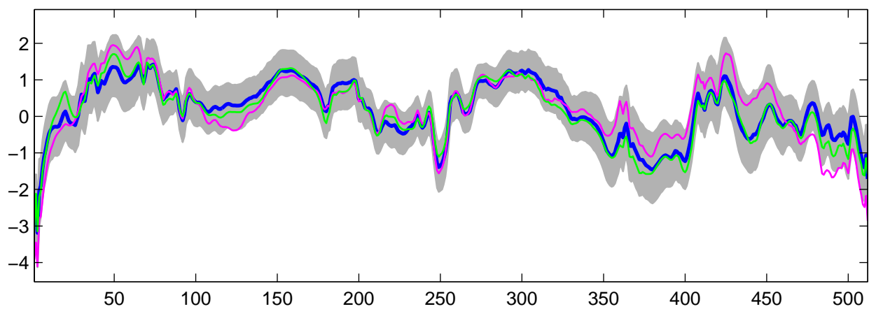
Estimated U_{11}(t) using R-WFMM: Normal data, run 2
