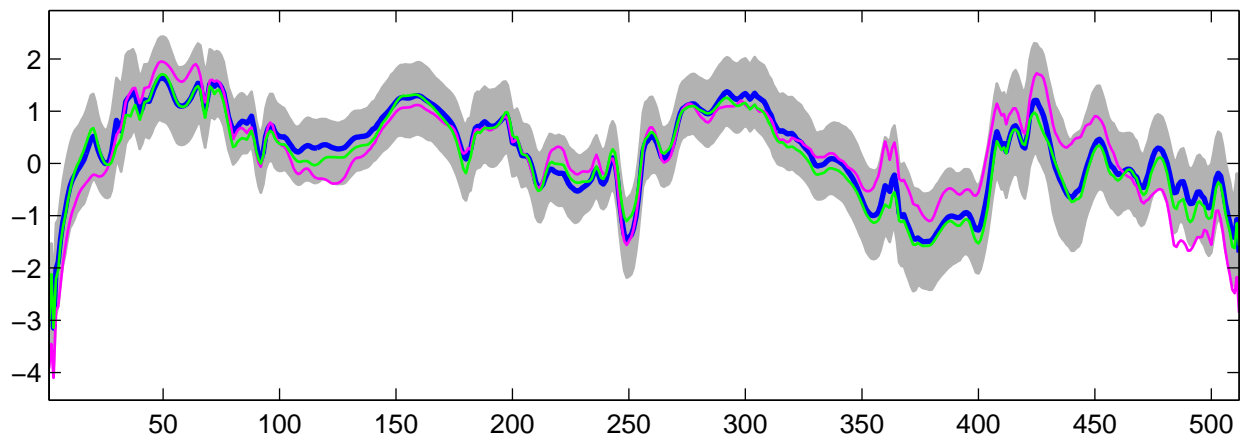
Estimated U_{11}(t) using G-WFMM: Normal data, run 2
