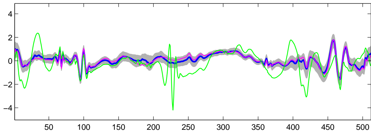
Estimated U_{11}(t) using R-WFMM: t_1 data, run 2
