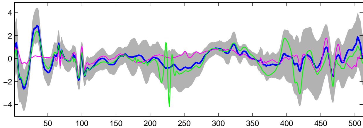
Estimated U_{11}(t) using G-WFMM: t_1 data, run 2
