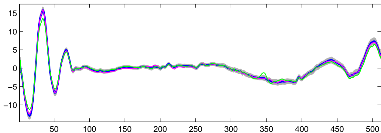
Estimated U_{11}(t) using R-WFMM: t_2 data, run 2
