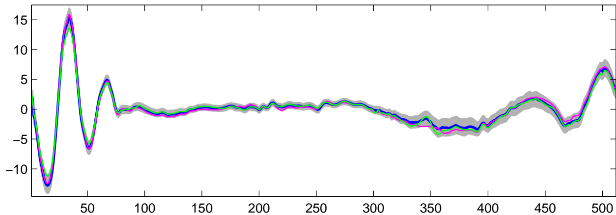
Estimated U_{11}(t) using G-WFMM: t_2 data, run 2
