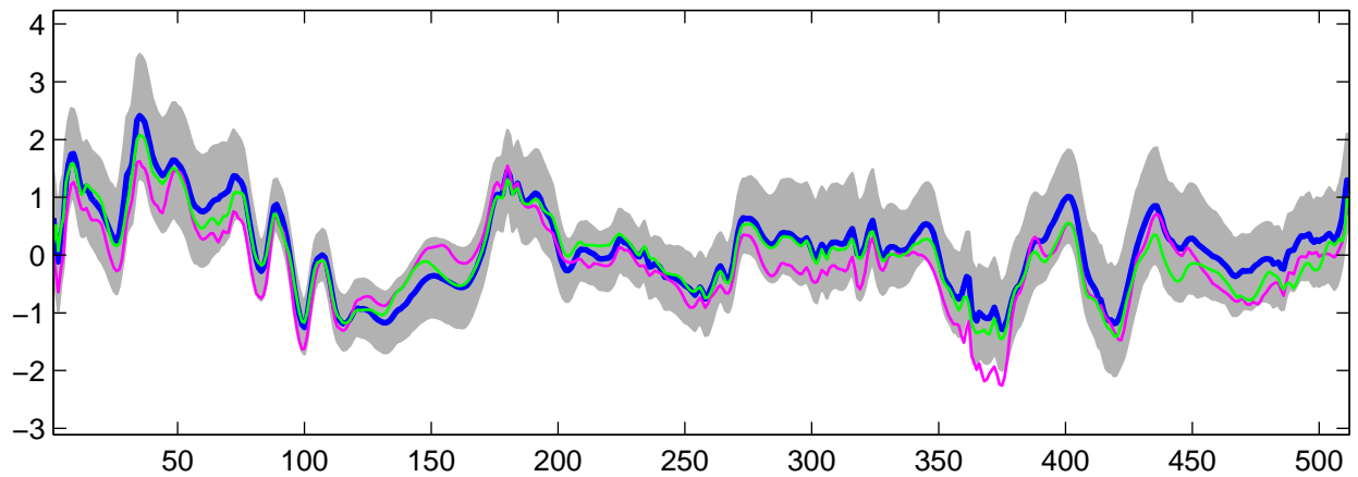
Estimated U_{12}(t) using R-WFMM: DE data, run 2
