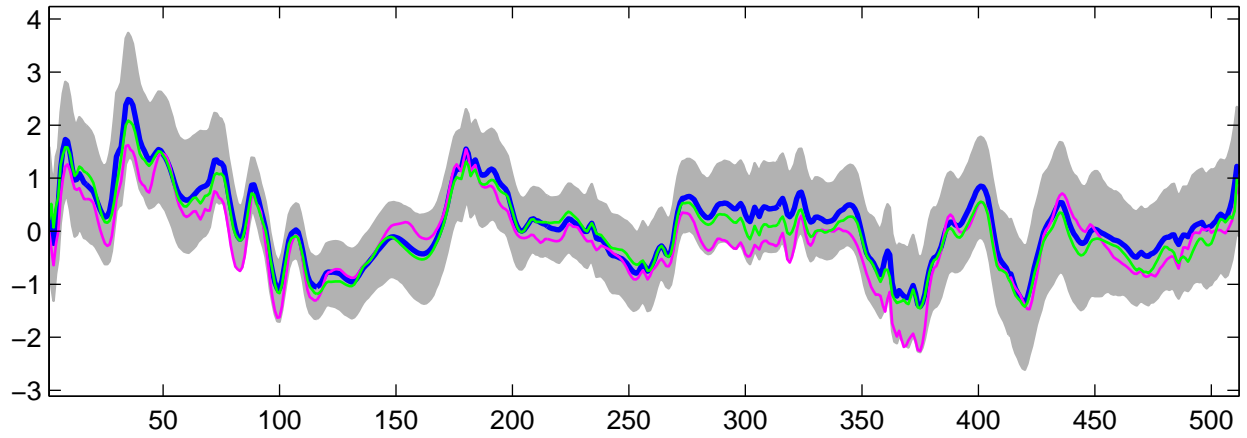
Estimated U_{12}(t) using G-WFMM: DE data, run 2
