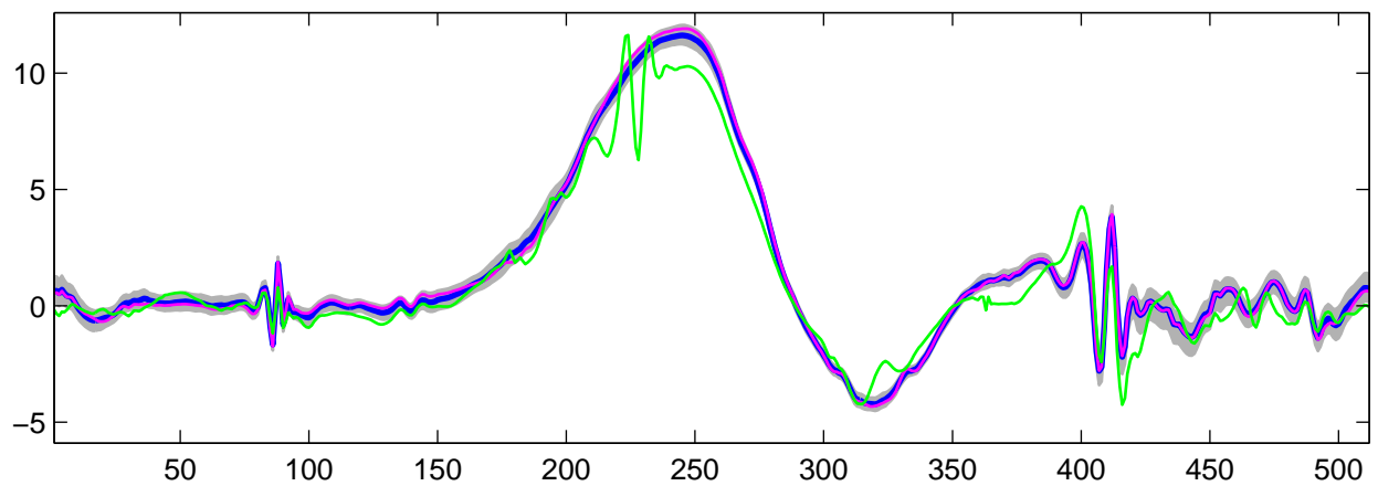
Estimated U_{12}(t) using R-WFMM: t_1 data, run 2
