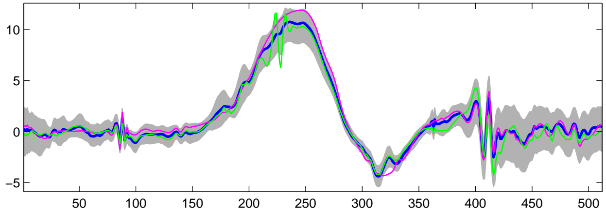
Estimated U_{12}(t) using G-WFMM: t_1 data, run 2
