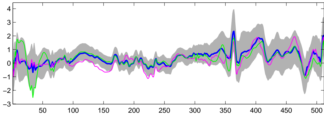
Estimated U_{12}(t) using G-WFMM: t_2 data, run 2
