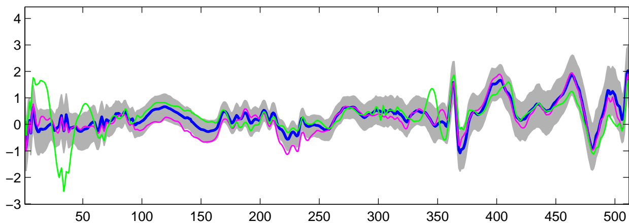
Estimated U_{12}(t) using R-WFMM: t_2 data, run 2
