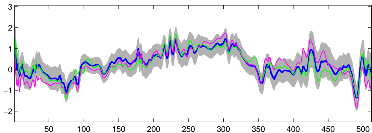
Estimated U_{12}(t) using R-WFMM: t_3 data, run 2
