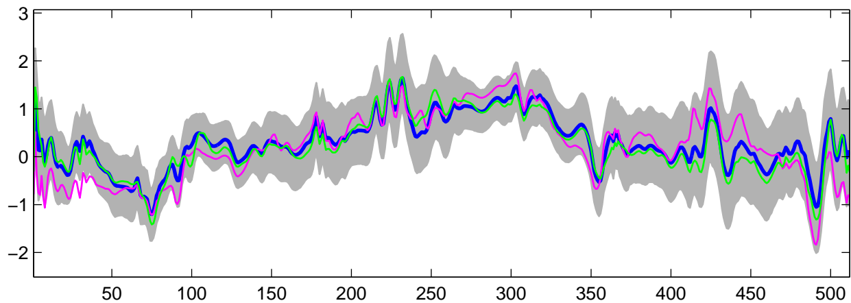
Estimated U_{12}(t) using G-WFMM: t_3 data, run 2
