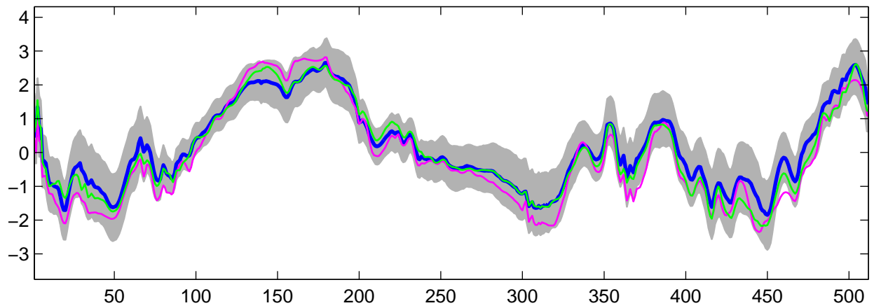
Estimated U_{13}(t) using R-WFMM: DE data, run 2
