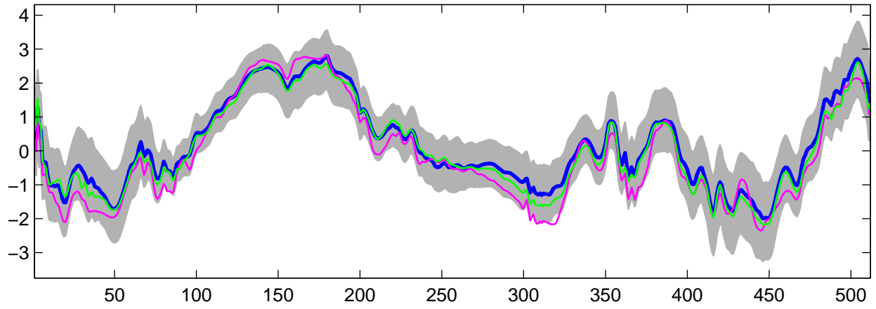
Estimated U_{13}(t) using G-WFMM: DE data, run 2
