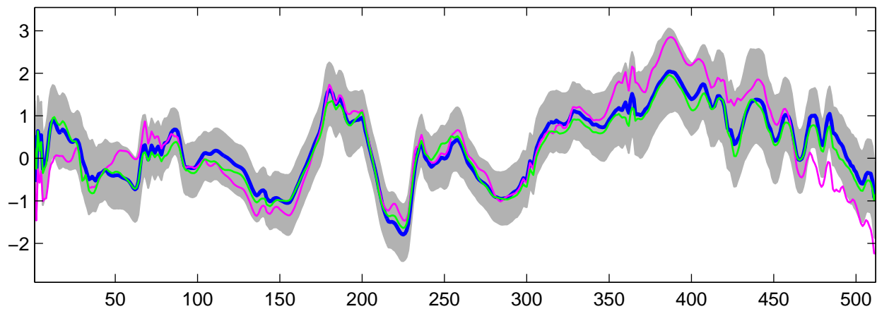
Estimated U_{13}(t) using G-WFMM: Normal data, run 2
