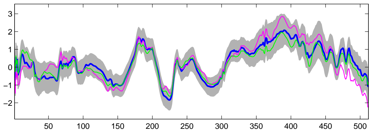
Estimated U_{13}(t) using R-WFMM: Normal data, run 2
