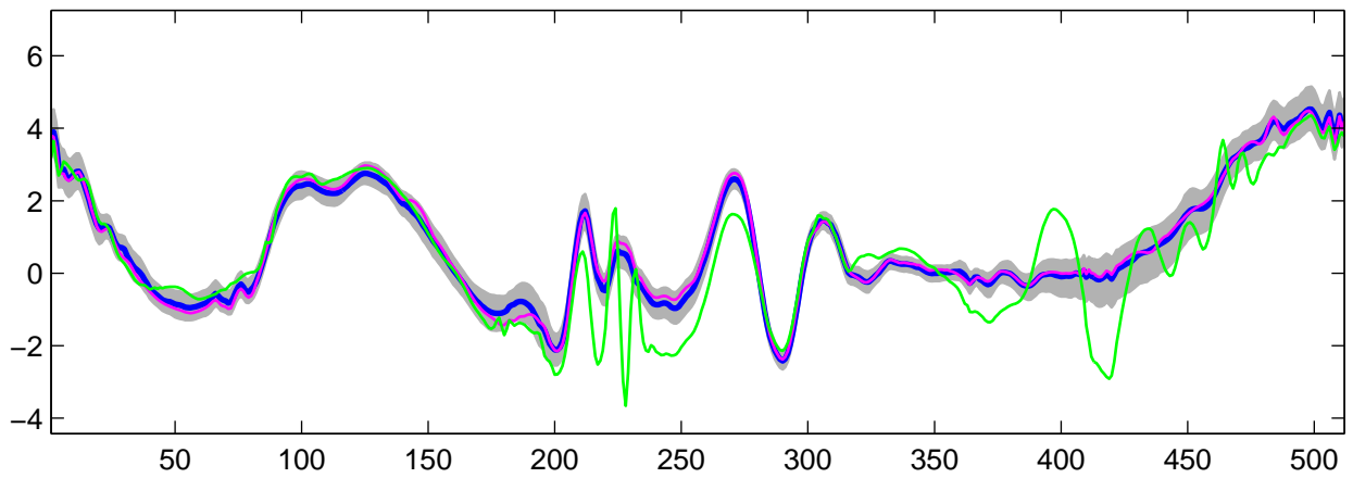
Estimated U_{13}(t) using R-WFMM: t_1 data, run 2
