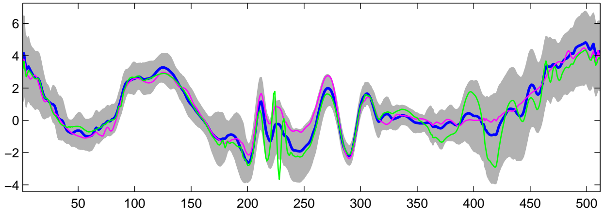
Estimated U_{13}(t) using G-WFMM: t_1 data, run 2
