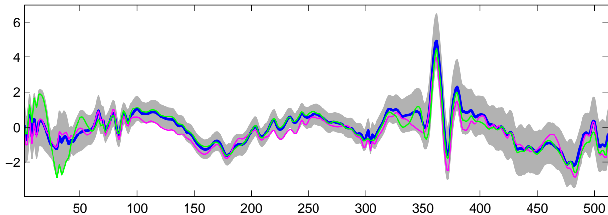
Estimated U_{13}(t) using G-WFMM: t_2 data, run 2
