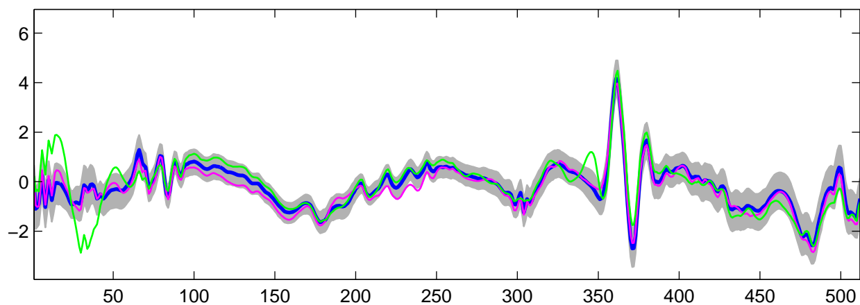
Estimated U_{13}(t) using R-WFMM: t_2 data, run 2
