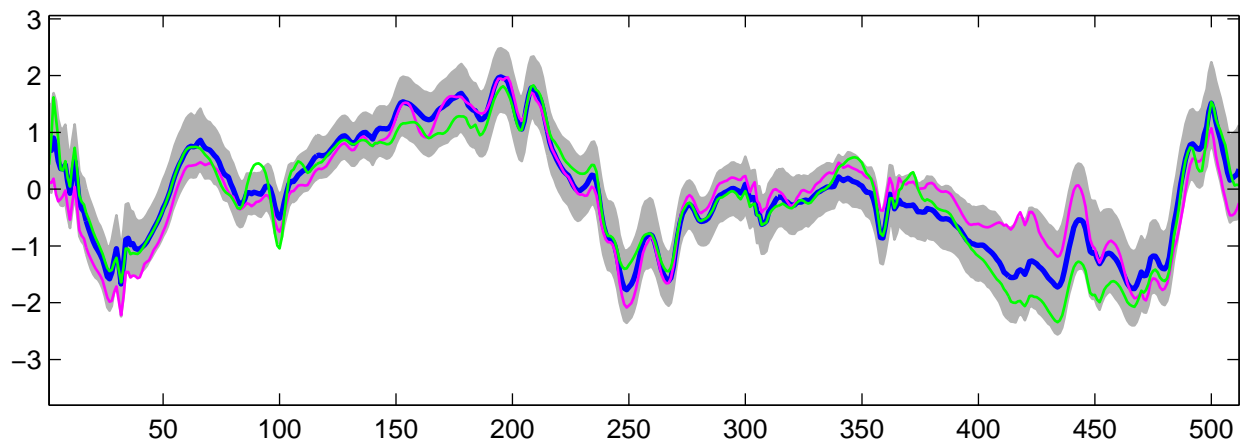
Estimated U_{13}(t) using R-WFMM: t_3 data, run 2
