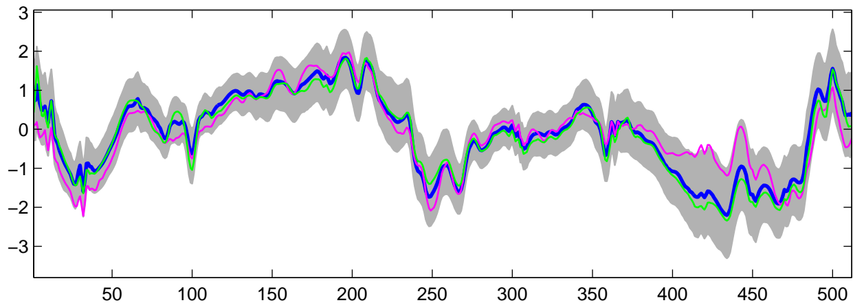
Estimated U_{13}(t) using G-WFMM: t_3 data, run 2
