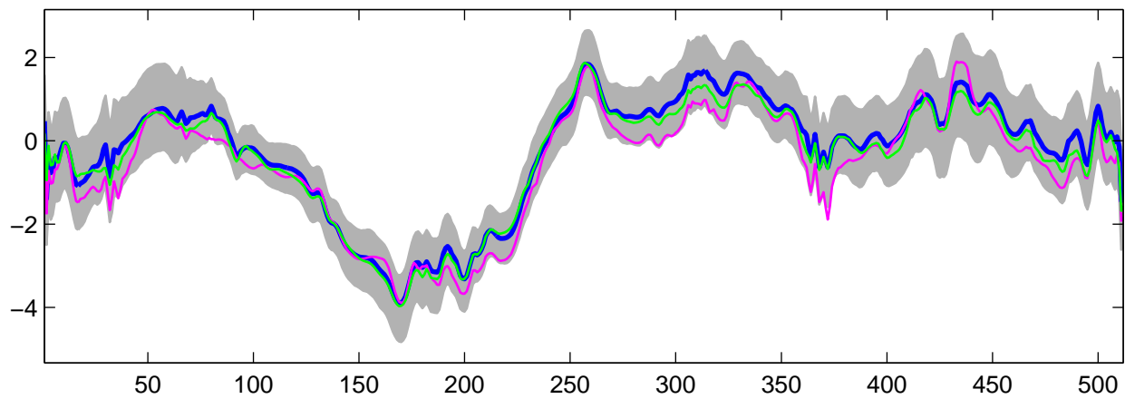
Estimated U_{14}(t) using G-WFMM: DE data, run 2
