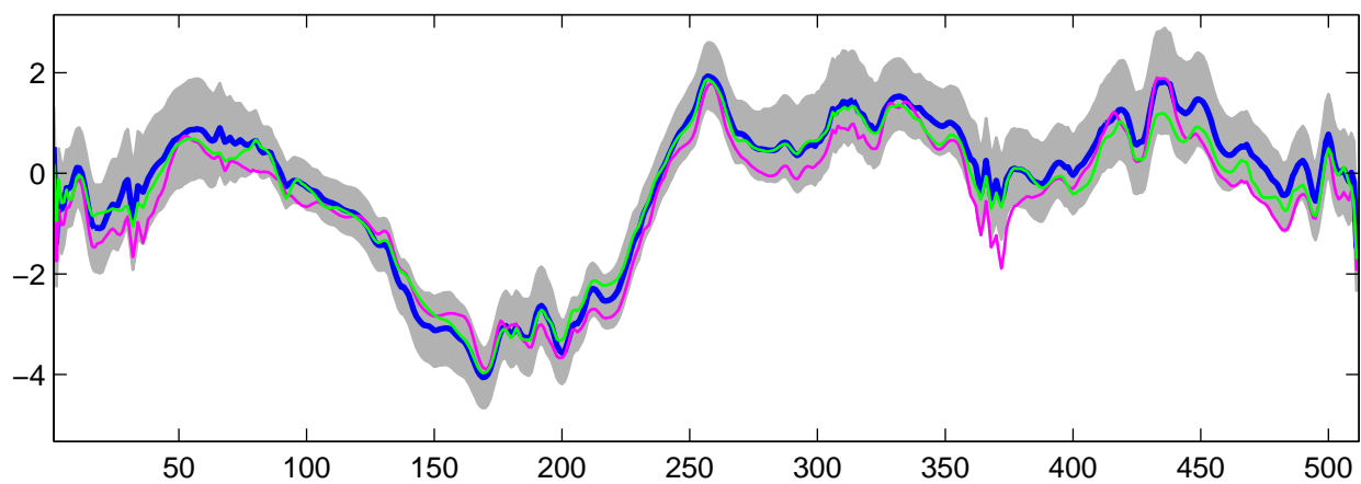
Estimated U_{14}(t) using R-WFMM: DE data, run 2
