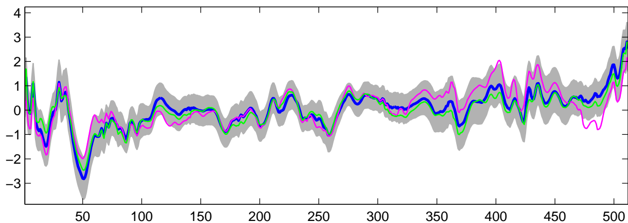
Estimated U_{14}(t) using R-WFMM: Normal data, run 2
