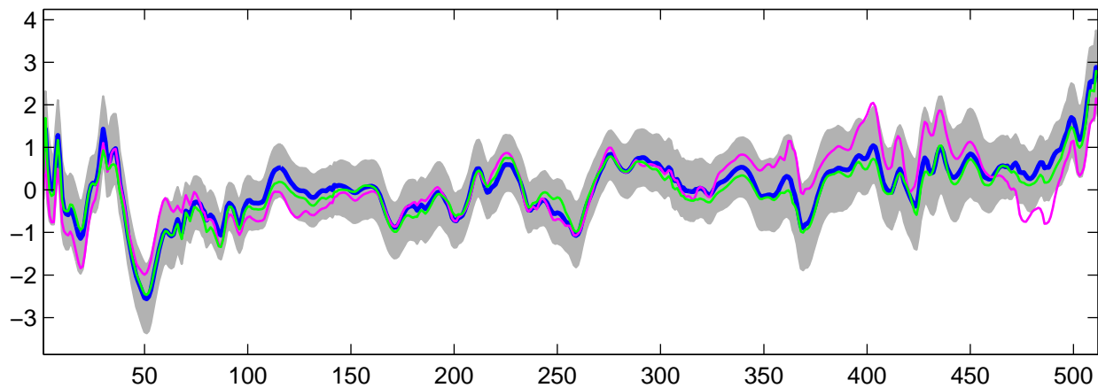
Estimated U_{14}(t) using G-WFMM: Normal data, run 2
