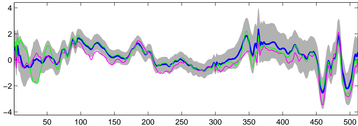
Estimated U_{14}(t) using G-WFMM: t_2 data, run 2
