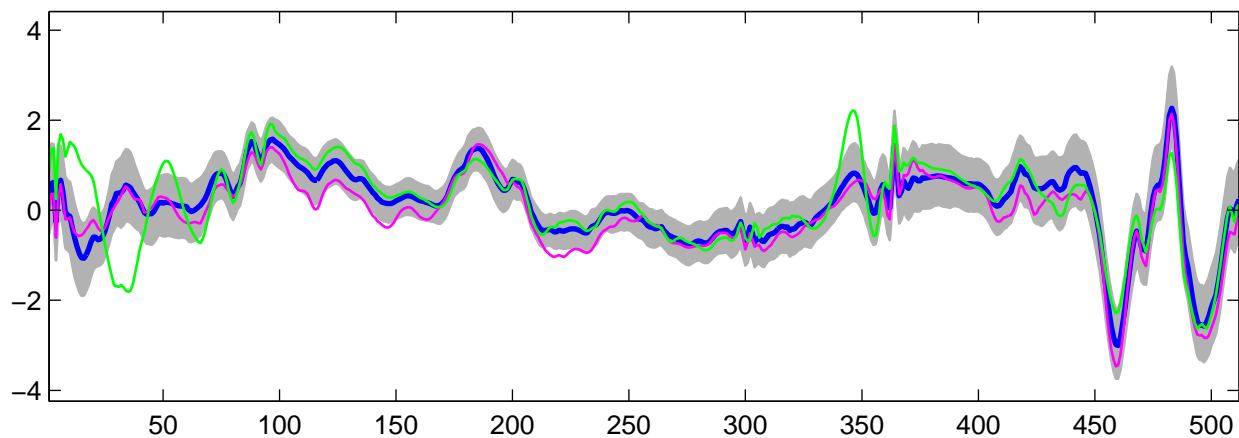
Estimated U_{14}(t) using R-WFMM: t_2 data, run 2
