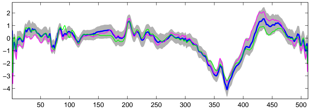
Estimated U_{14}(t) using R-WFMM: t_3 data, run 2
