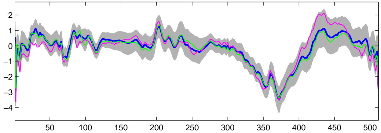
Estimated U_{14}(t) using G-WFMM: t_3 data, run 2
