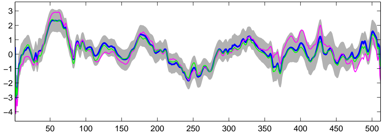
Estimated U_{15}(t) using G-WFMM: Normal data, run 2
