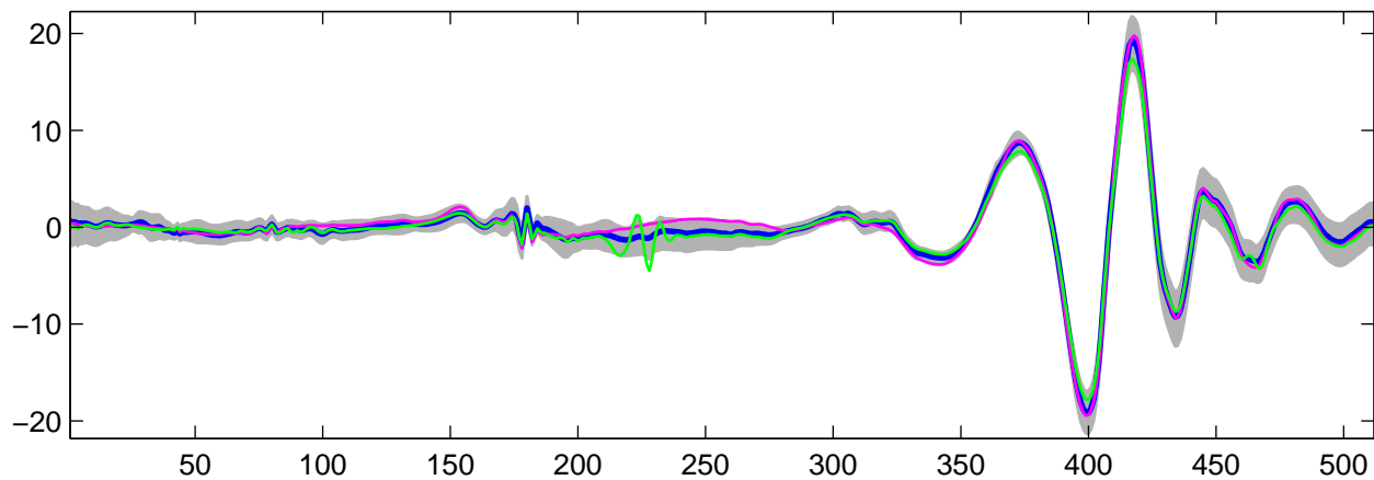
Estimated U_{15}(t) using G-WFMM: t_1 data, run 2
