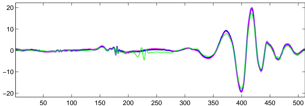
Estimated U_{15}(t) using R-WFMM: t_1 data, run 2
