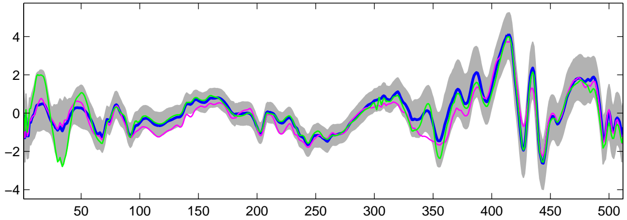
Estimated U_{15}(t) using G-WFMM: t_2 data, run 2
