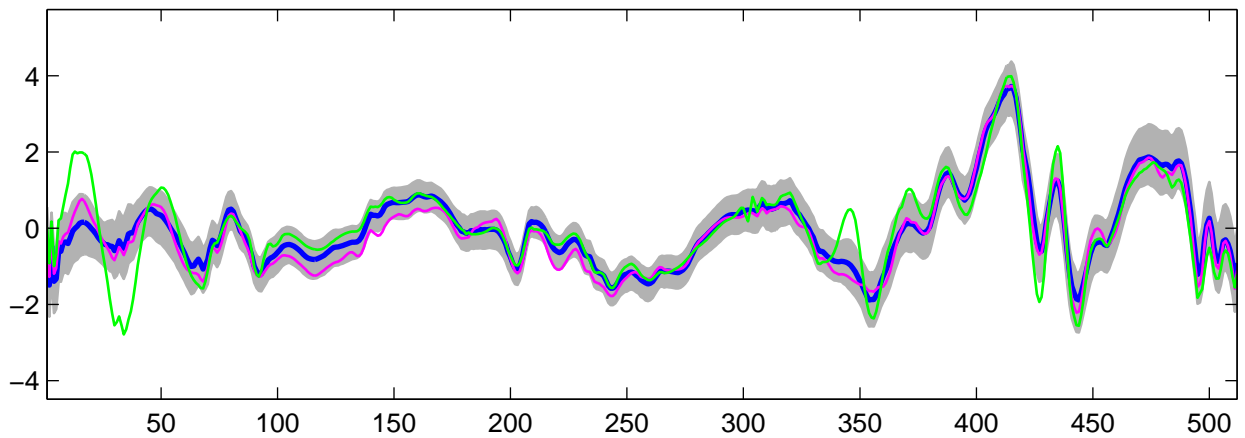
Estimated U_{15}(t) using R-WFMM: t_2 data, run 2
