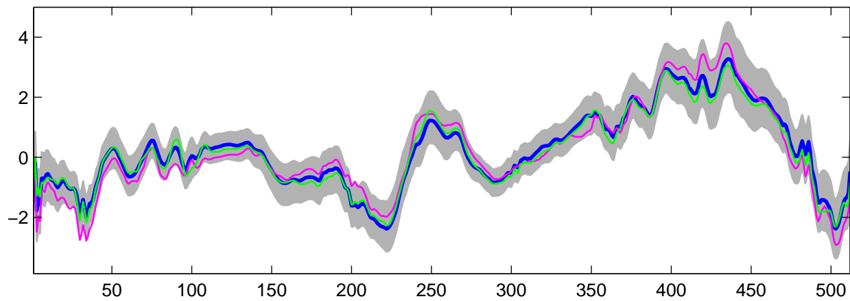
Estimated U_{15}(t) using G-WFMM: t_3 data, run 2
