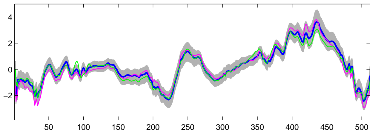
Estimated U_{15}(t) using R-WFMM: t_3 data, run 2
