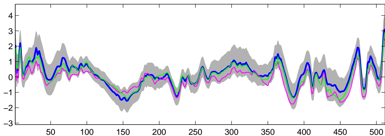
Estimated U_{16}(t) using R-WFMM: DE data, run 2
