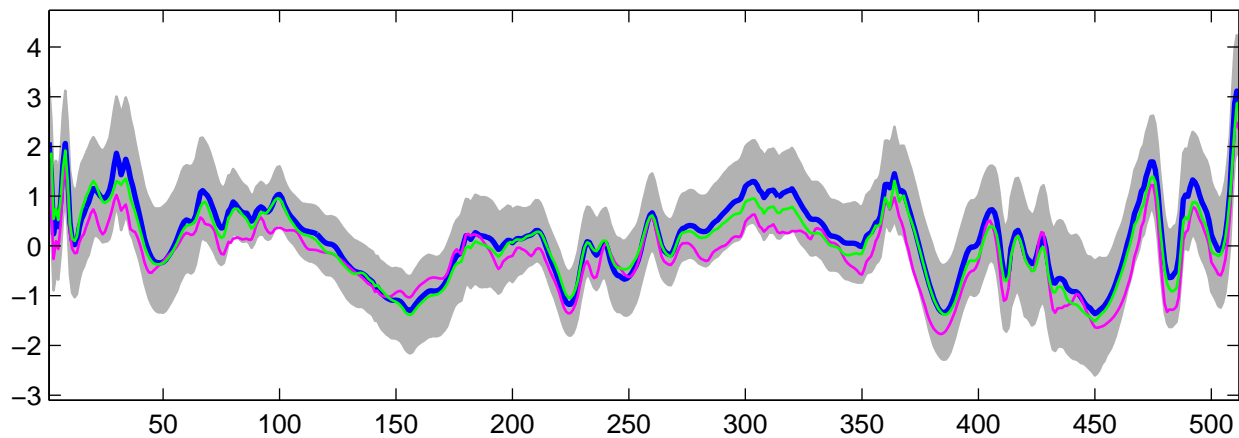
Estimated U_{16}(t) using G-WFMM: DE data, run 2
