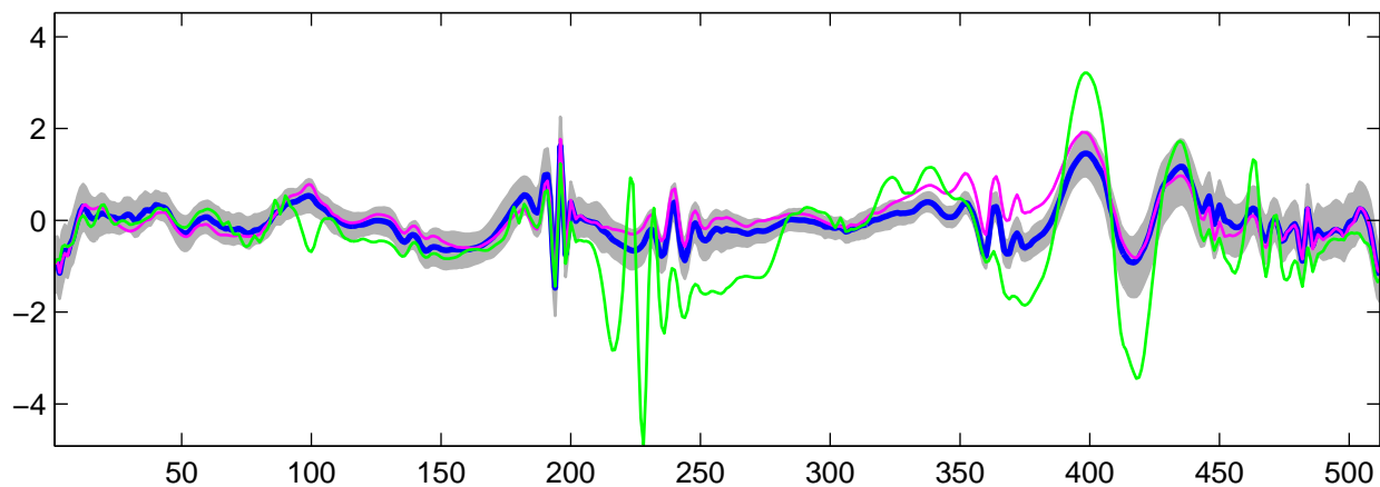
Estimated U_{16}(t) using R-WFMM: t_1 data, run 2
