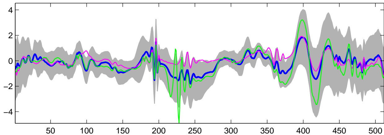
Estimated U_{16}(t) using G-WFMM: t_1 data, run 2
