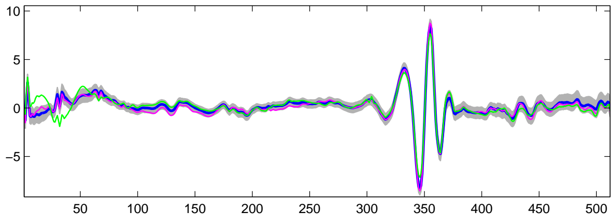
Estimated U_{16}(t) using R-WFMM: t_2 data, run 2
