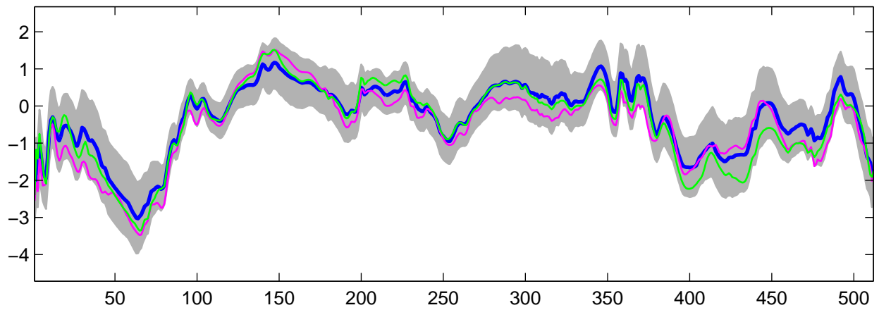
Estimated U_{17}(t) using R-WFMM: DE data, run 2
