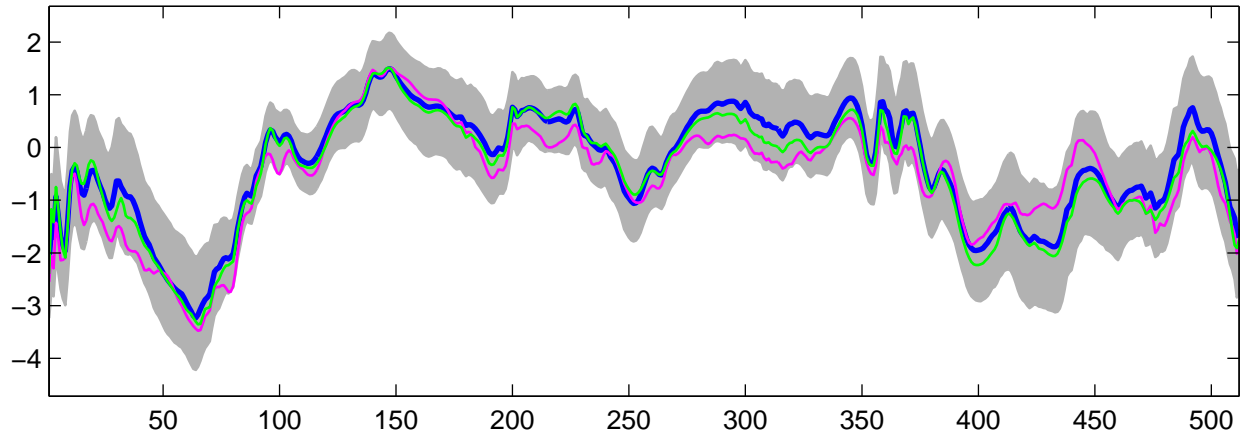
Estimated U_{17}(t) using G-WFMM: DE data, run 2
